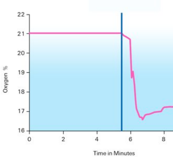
Graph 1. Reduction of oxygen concentration from 21% to 16.8% at the flame front during high pressure water discharge.
