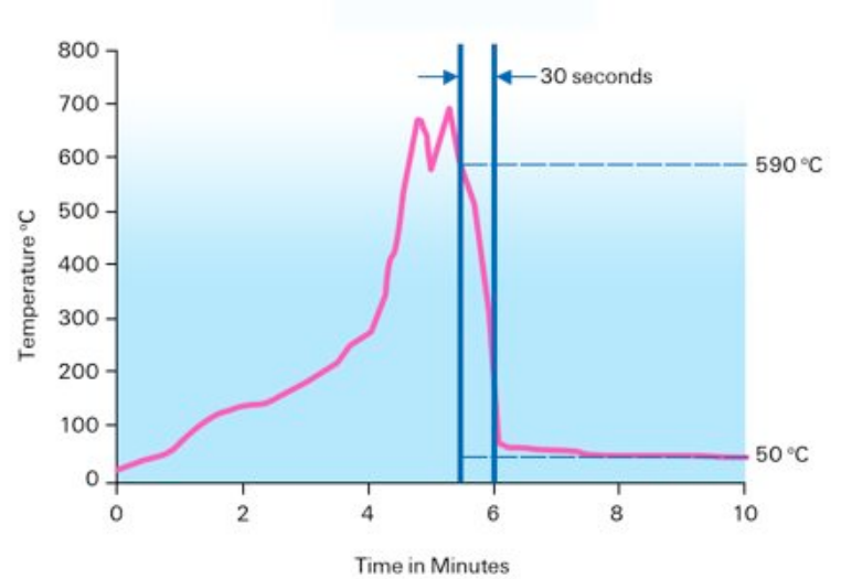
Graph 2. Reduction of temperature from 590°C to 50°C during initial 30sec of discharge (preburn time before manual operation).
